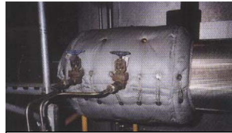
High Pressure Orifice Flange
